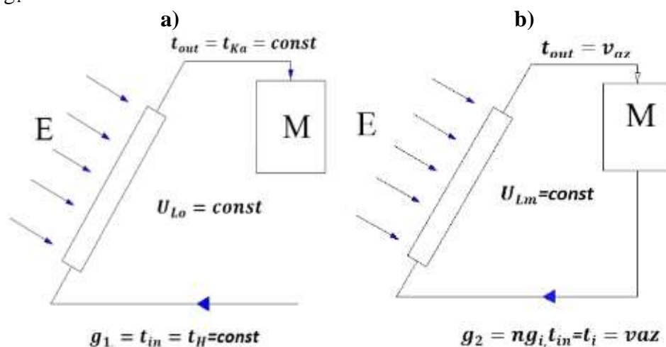
Fig. 1. Diagram of solar collector operation in (a) single –and (b) multiple-heating regimes.
